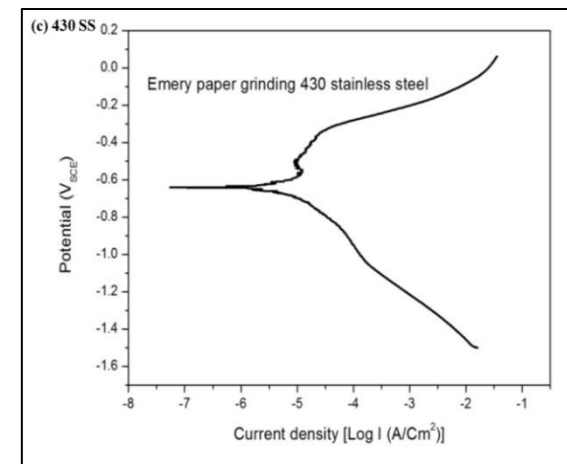
Fig 5(c): The Experimental Polarisation Curve of 430 Stainless Steel Sample
