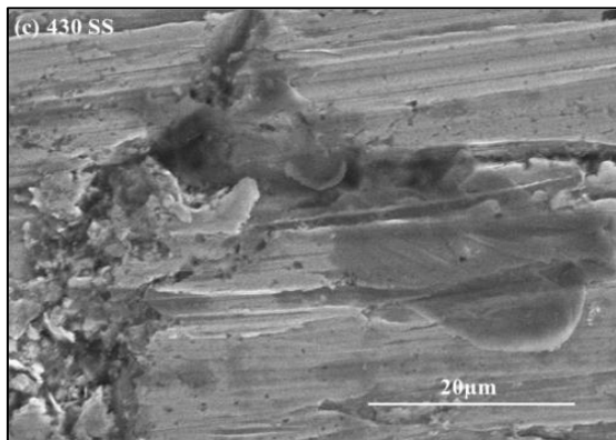
Fig 6(c): Emery Paper Grinding Corroded Sample of 430 Stainless Steel Sample
