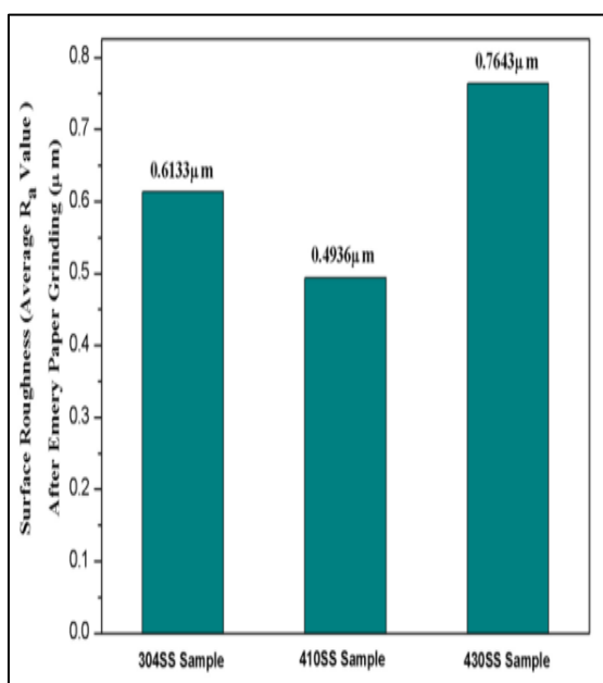
Fig. 2. Surface Finish Data are Presented in Bar Diagram form
