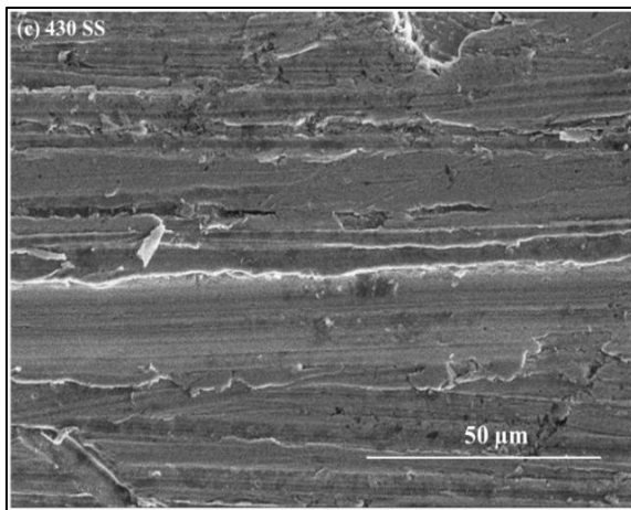
Fig 4(c): 430 Stainless Steel Sample Sem Photographs Of emery Paper Grinding
